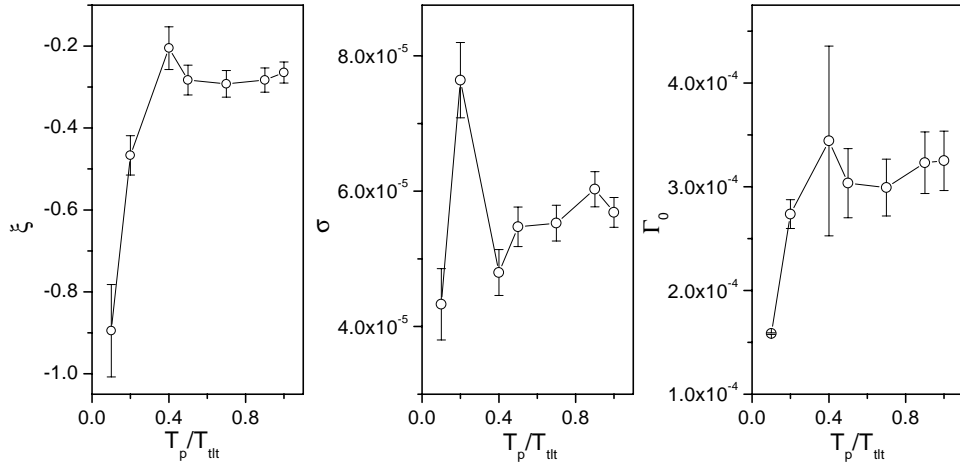
Figure 9. Parameters fitted from short-term and long-term series at the station x=7.8D , GLS. Bars: \xi and \sigma , standard error; \Gamma_0 , 95% confidence interval. T_{lt} total duration, T_p short duration.
