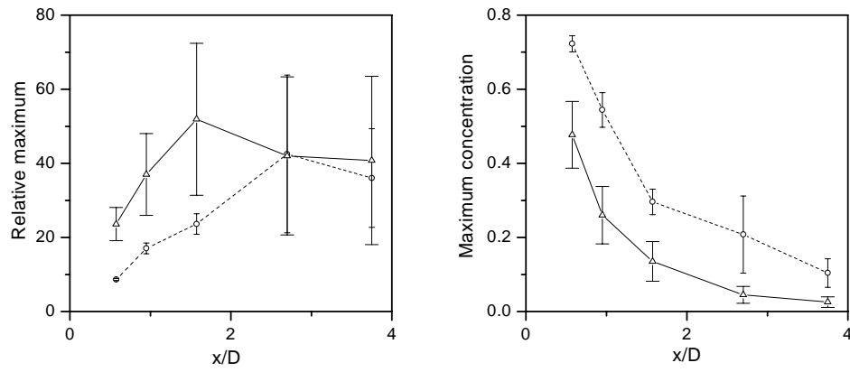
Figure 11. Source size effect on maximum concentration. Vertical bars: 95% confidence intervals; \text{---}\triangle\text{---} normal size; \text{---}\circ\text{---} bigger size. Left: relative maxima, \Gamma_0(x)/C_m(x) . Right: maxima normalized by source concentration, \Gamma_0(x)/C(0) .
