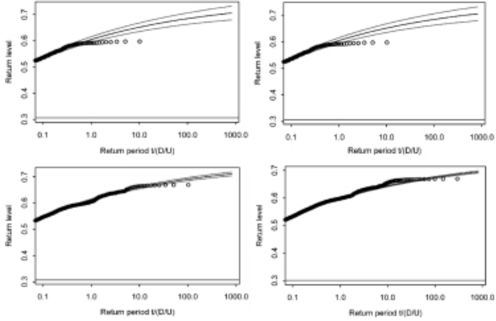
Figure 8. Return level extrapolation. LES, very coarse mesh; from left to right, then top to bottom, 10^4 , 10^5 , 10^6 , 3 \times 10^6 time steps respectively. Circles, LES data. Lines, EVT predicted with 95% confidence intervals.
