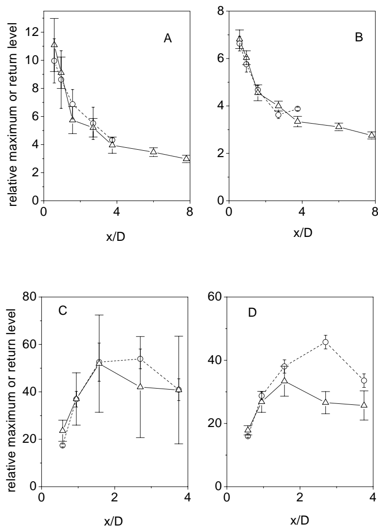
Figure 10. Relative maxima and return levels. Bars: 95% confidence intervals; \text{---}\triangle\text{---} LES; \text{---}\circ\text{---} measurements. A: GLS, relative maxima; B: GLS, return level for return period of 3.6 times of whole LES duration; C and D: ES, as A and B respectively.
