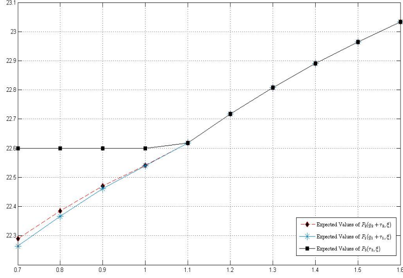
Figure 3: Comparative static analysis on the expected node prices with respect to the change of \beta_1 .
