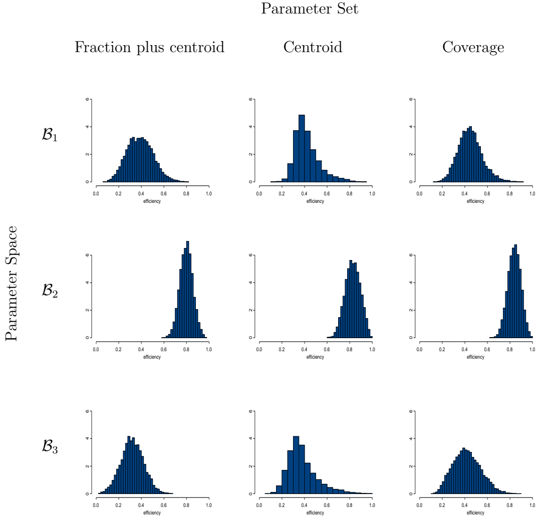
Figure 2: Distributions of efficiencies of nine compromise designs for three parameter spaces and three parameter sets.
