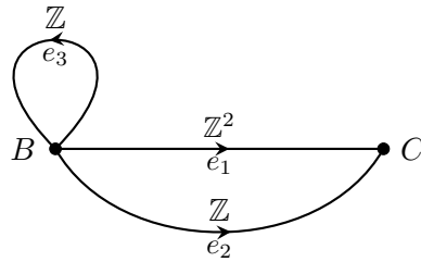
FIGURE 2. The graph of groups (\mathcal{G}, \Gamma) in Example 10.2
